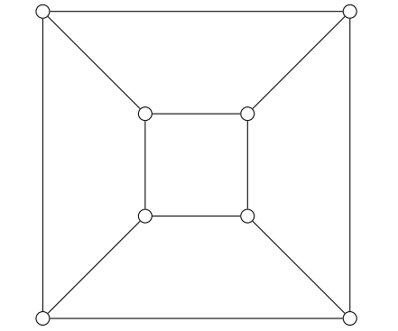
(b) Planar bipartite 2-vertex-connected subcubic (undirected).
