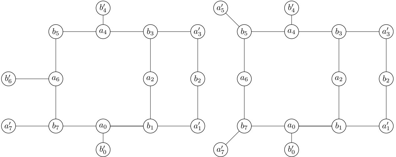
Figure 12: Configurations of Lemma 30
