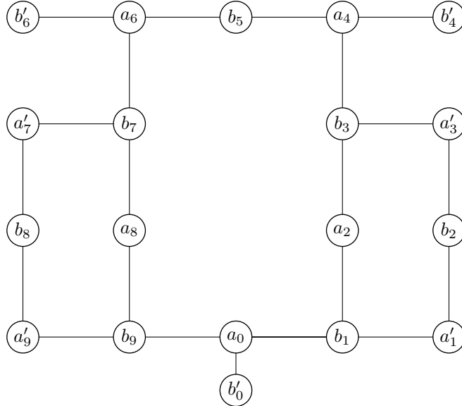
Figure 13: Configuration in Lemma 31
